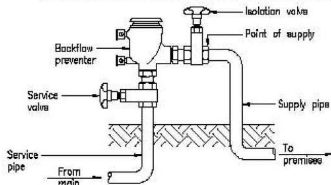
Figure: UNMETERED SUPPLY WITH VACUUM BREAKER BACKFLOW PREVENTER
