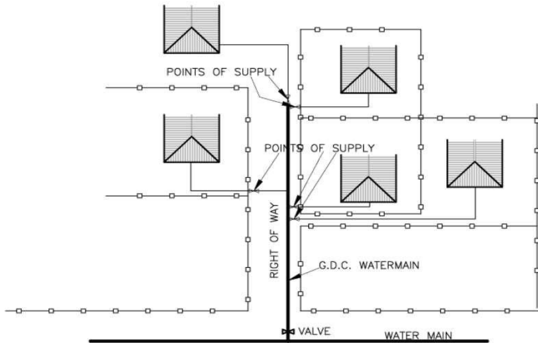
EXAMPLE 3: REAR LOTS ON RIGHT OF WAY (5 OR MORE CUSTOMERS) POINT OF SUPPLY OUTSIDE PROPERTY N.T.S.
