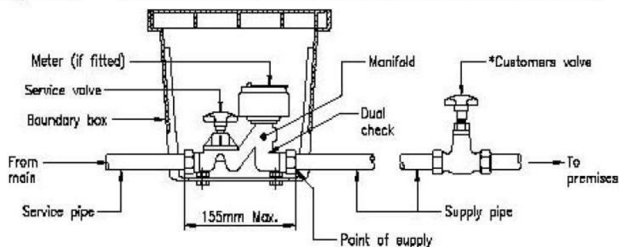
Fig. 7a MANIFOLD ASSEMBLY AT BOUNDARY BOX
