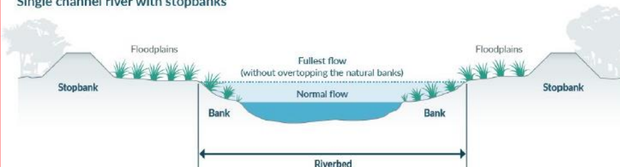
Single channel river with stopbanks
