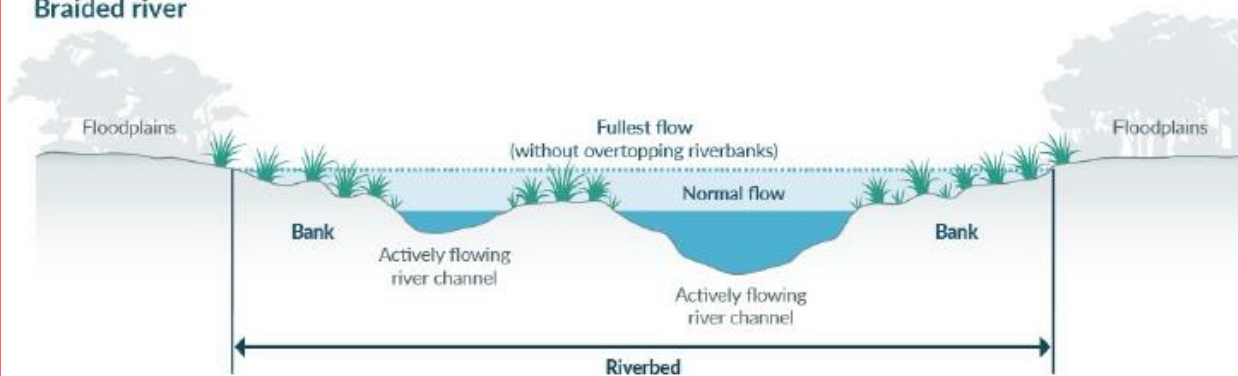
Braided river
